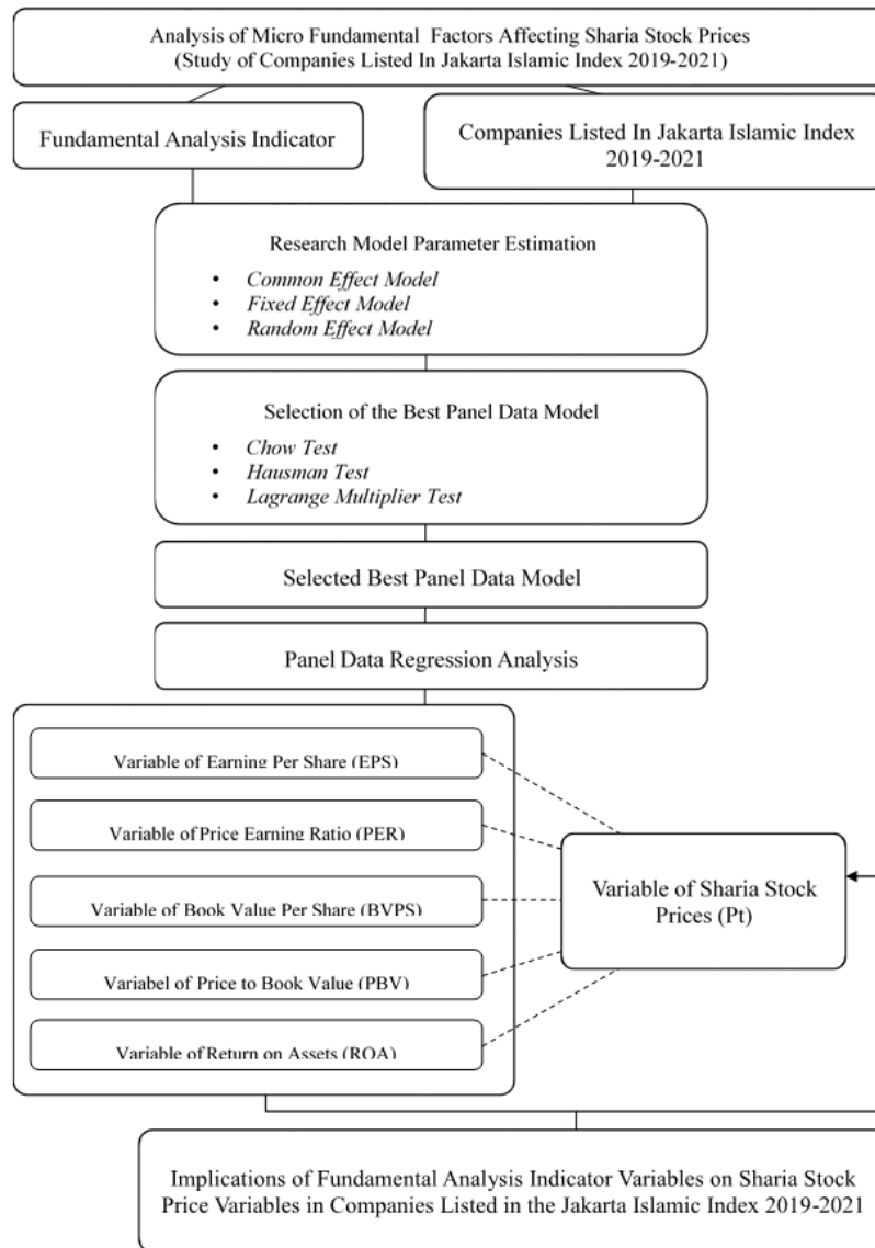
Figure 1. Framework Research
