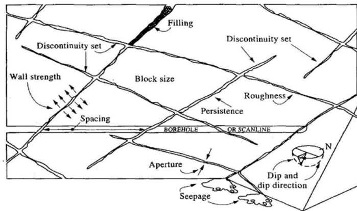
Figure 1. Geometric Properties of Discontinuities (Hudson & Priest, 1979)
